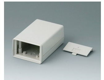
A9406344 BOITIER COQUILLES V 110, Vers. II ABS (UL 94 HB) gris blanc RAL 9002 72x114x45mm
